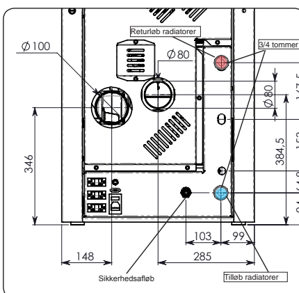
Fig. 12-B HRV160 / HR200
